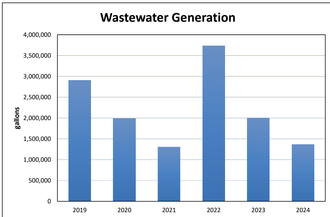
Figure 5.4.1-1 Wastewater Generation
